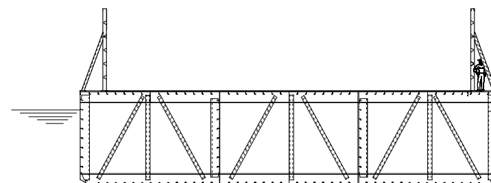
MIDSHIP SECTION
