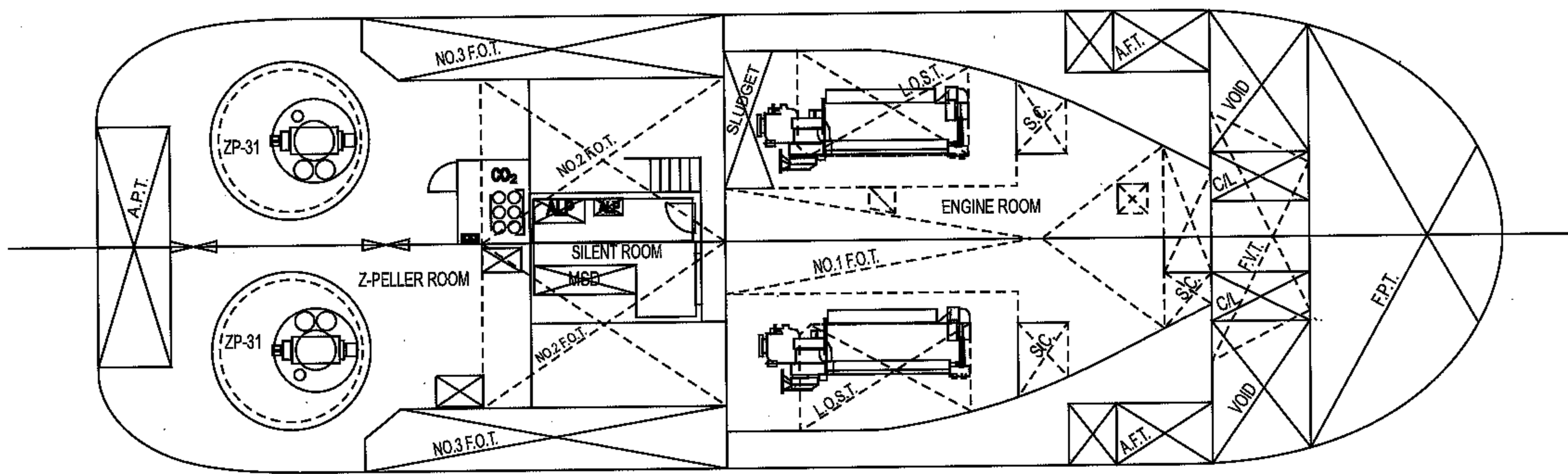
BOTTOM PLAN
