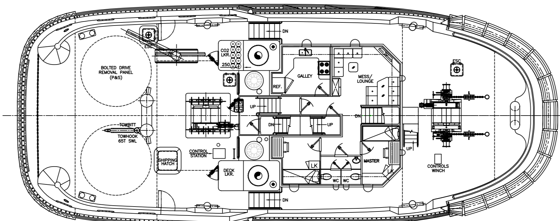
MAIN DECK PLAN
