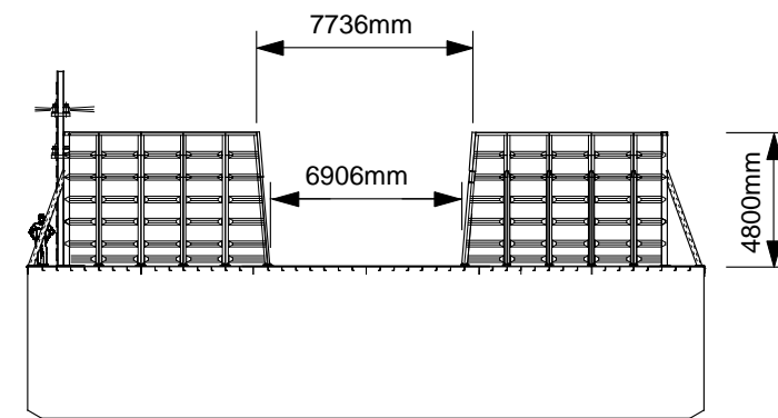
SECTION AT REMOVABLE AFT HOPPER WALL
