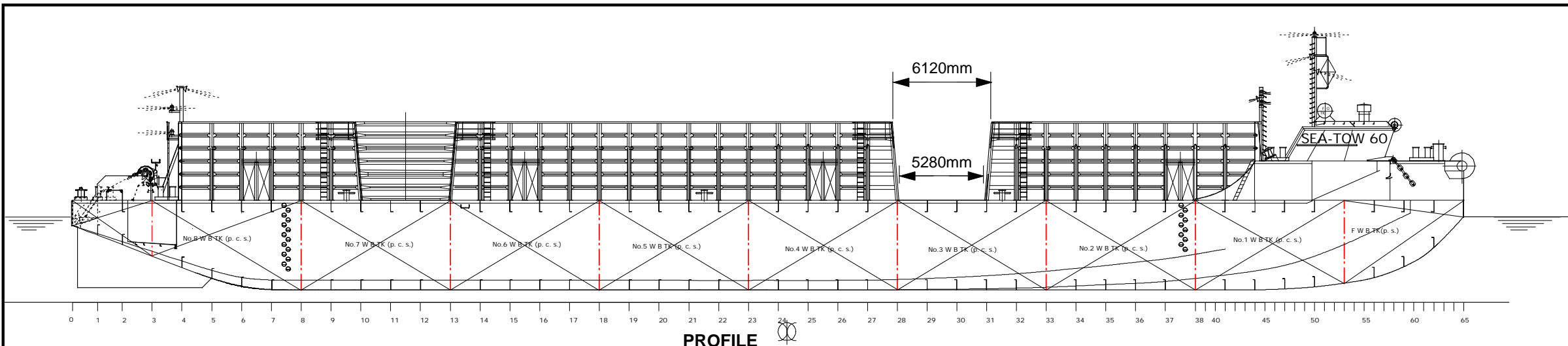
PROFILE
