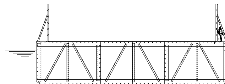
MIDSHIP SECTION
